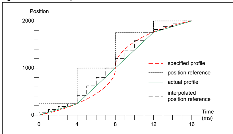
Figure 11-9 Linear interpolation
