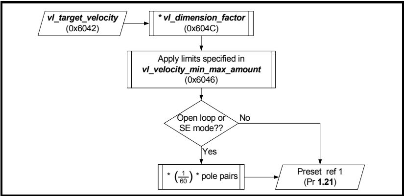
Figure 12-6 vl_target_velocity
