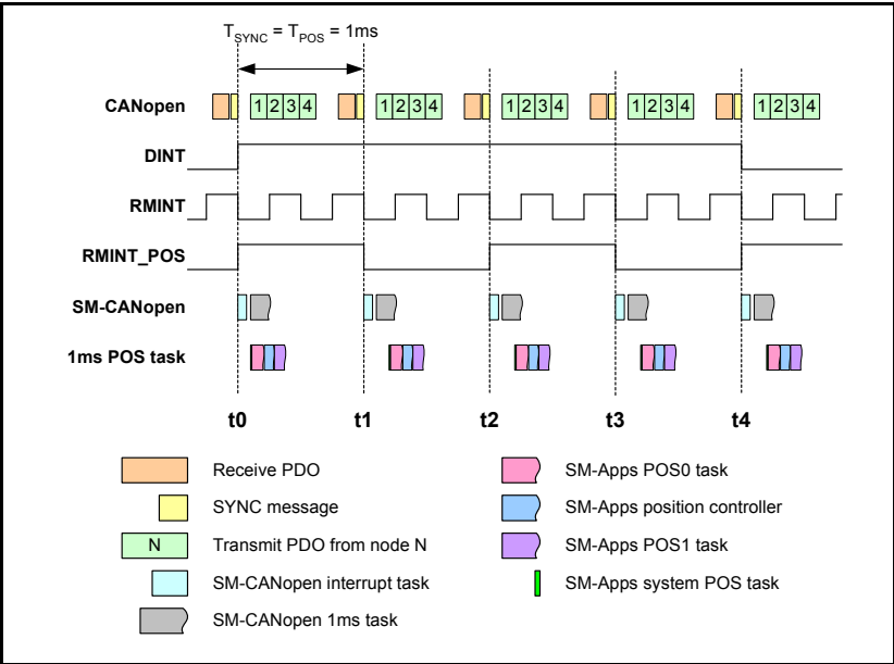
Figure 11-6 Example profile 1
