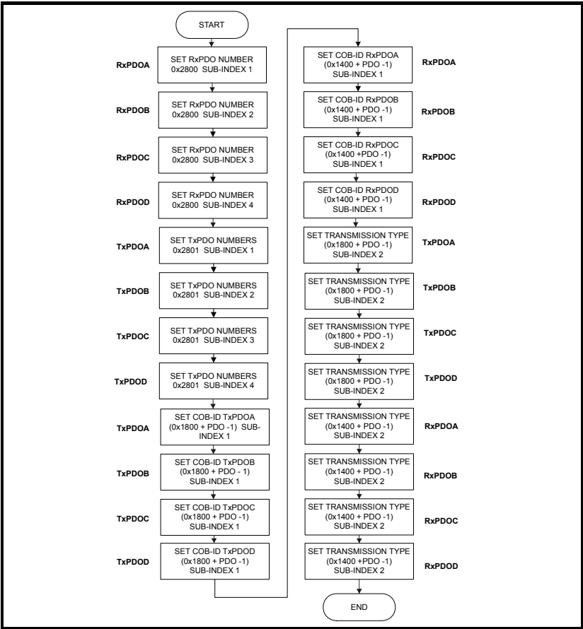
Figure 5-10 SDO Configuration
