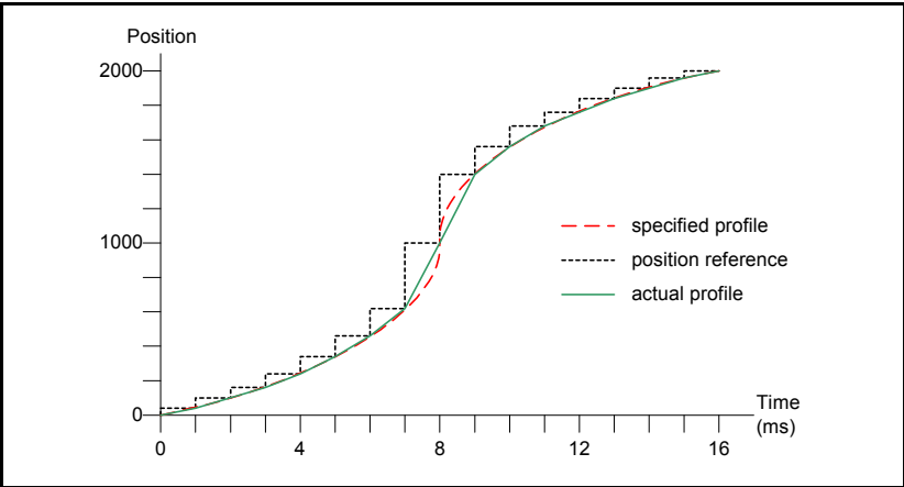
Figure 11-6 Example profile 1
