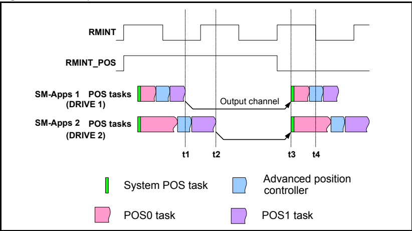
Figure 11-12 Output channel
