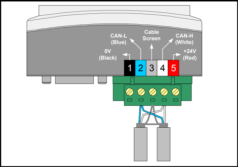
Figure 4-2 SM-CANopen connections
